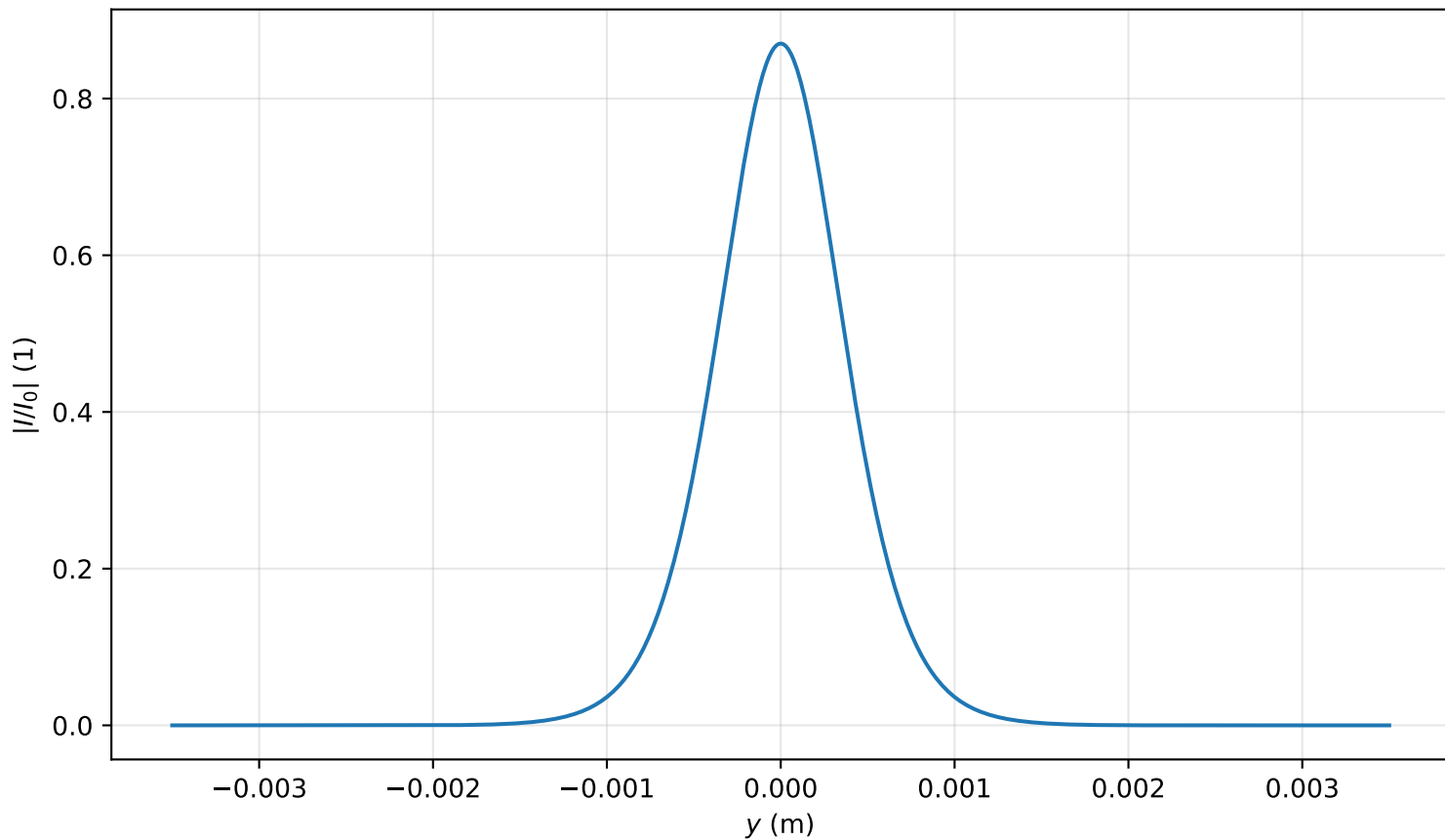
Intensity profile I(x=0, y, z=1.831)/I_0 , P_{in}=0.5P_{cr} , artificial time
